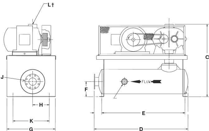
PneuPak "C" Package with discharge silencer
